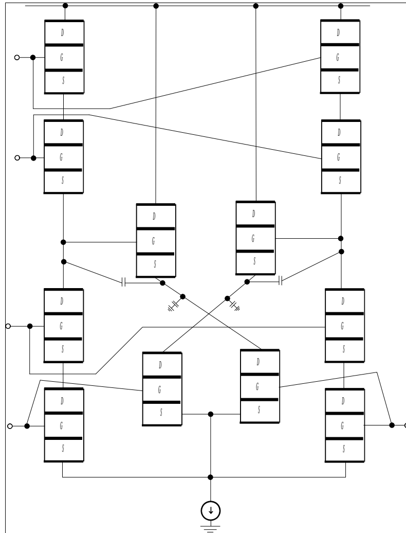
Fig 1a: Structure of the considered amplifier [19]
