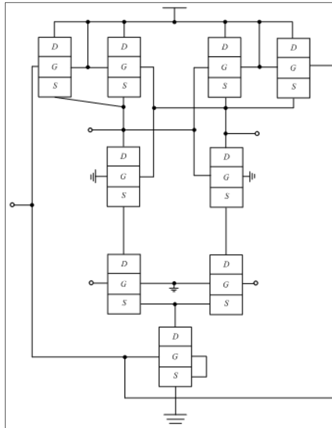
Fig 1a: Structure of the considered dynamic comparator [24]
